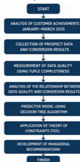
Figure 1. Research Framework
